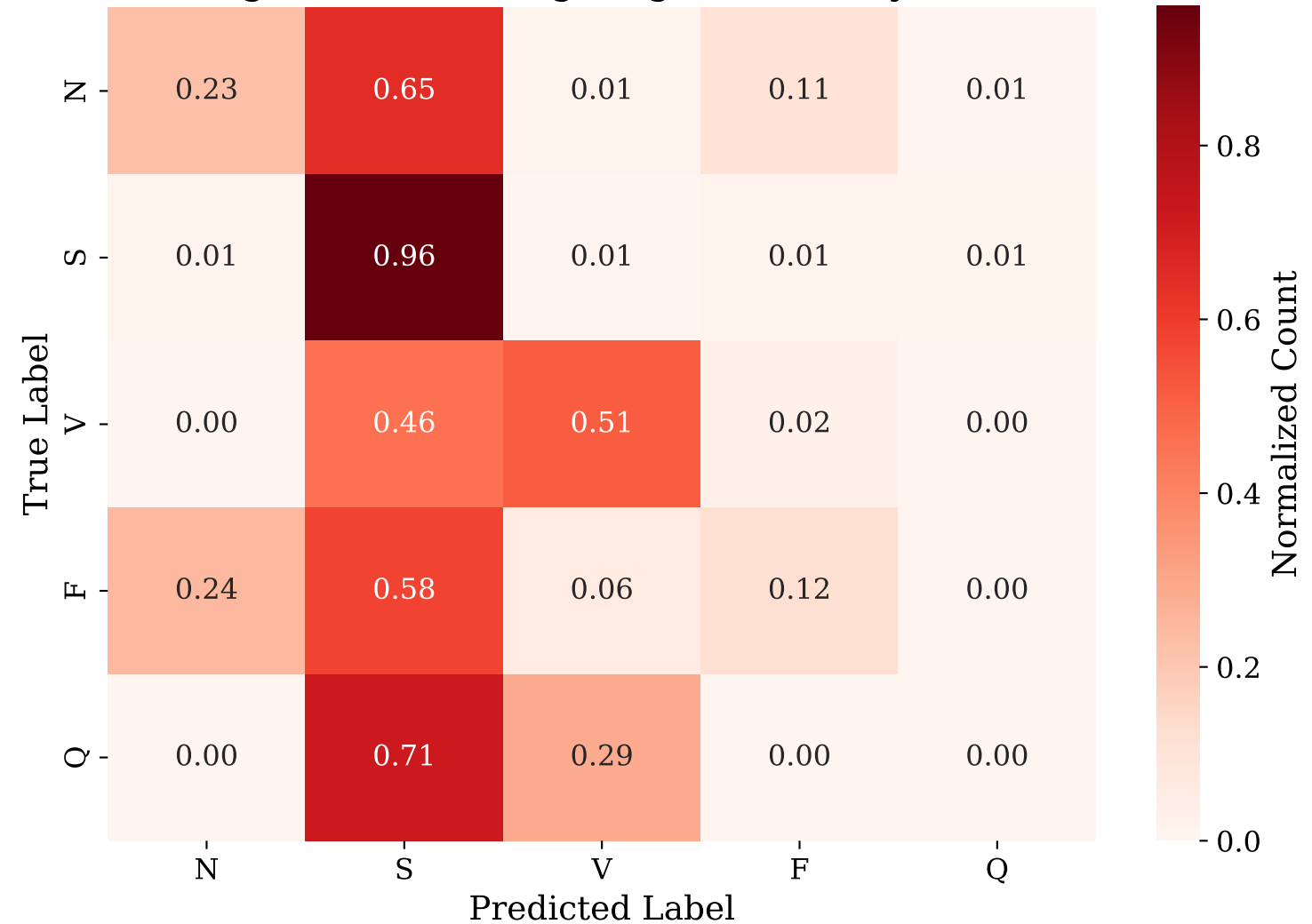
Disagreement Mining (High-Sensitivity Mode)
